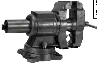
MV10 Head Rotates 360° for Standard or Pipe Jaw Vise. Head Locks Automatically.
